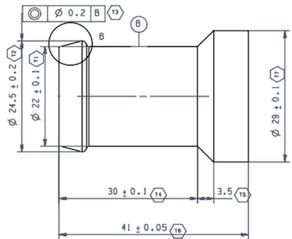
▪ Outlet Extension Pipe- C90 Series
